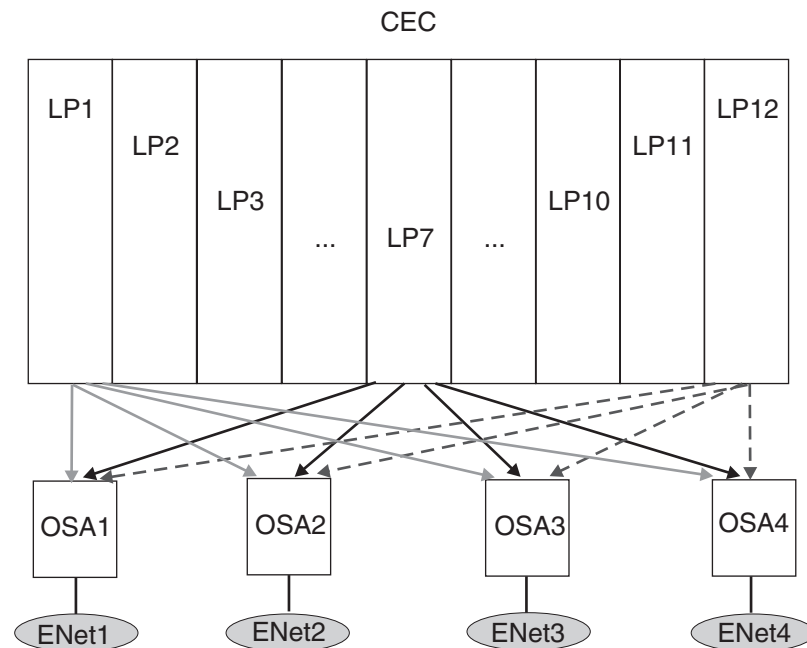
Figure 30. Candidate configuration for HiperSockets Accelerator
